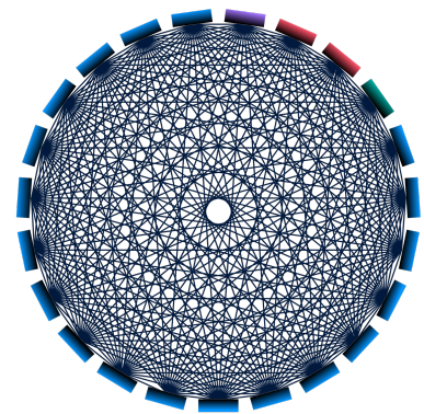
Figure 4.1: Dragonfly+ Topology. Booster Module nodes (blue), I/O cell (purple), Data-centric cells (red), and Hybrid cell (green) [cinecaLeonardoSystem].
